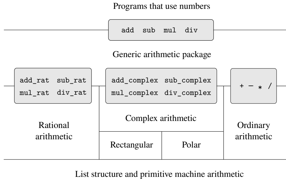
Figure 2.23 Generic arithmetic system.
