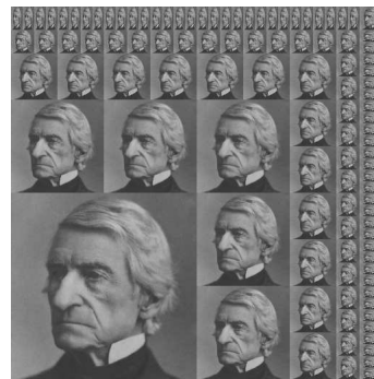
corner_split(rogers, 4)
