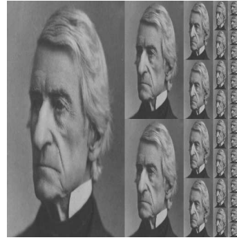
right_split(rogers, 4)
