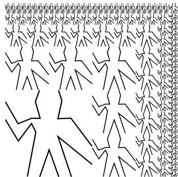
corner_split(wave, 4)
