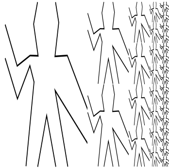
right_split(wave, 4)
