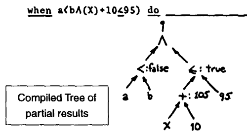
FIGURE 11.13 Flex when statement [Kay 1969]
