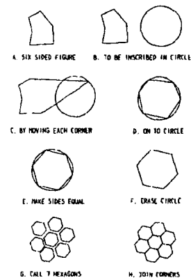
FIGURE 11.4 Drawing in Sketchpad
