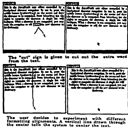
FIGURE 11.60 The author's pen-based interface for ST-
