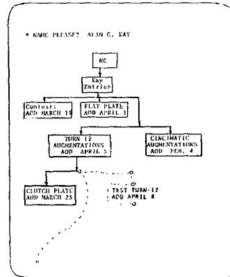
FIGURE 11.16 FLEX user interface. "Files" as suspended processes [Kay 1969]
