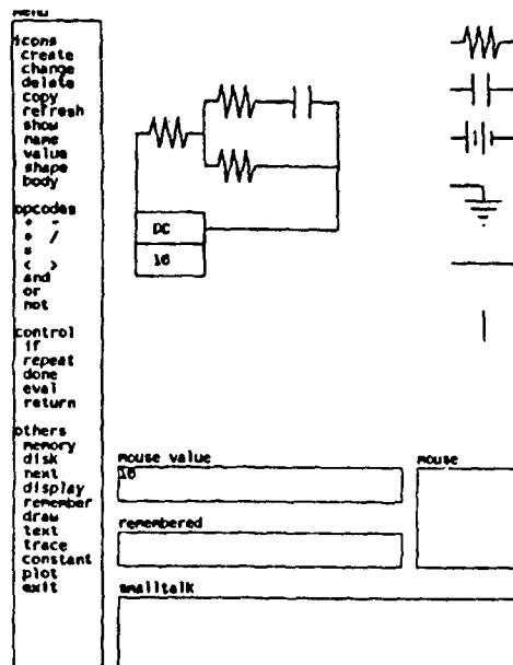
FIGURE 11.40 PYGMALION iconic programming
